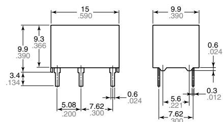
External dimensions
